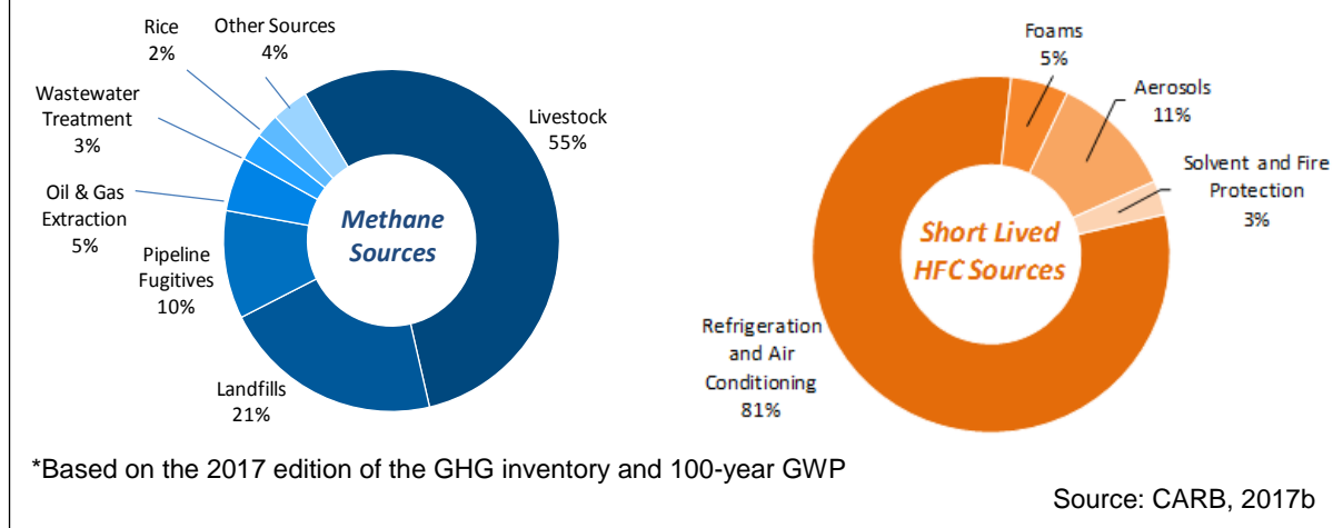
Figure 10. 2015 Sources of short-lived climate pollutants*
