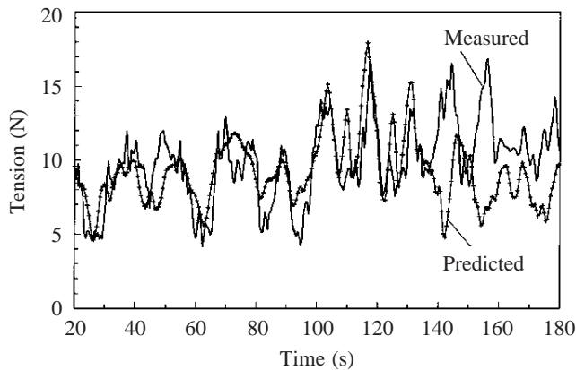
Fig. 5. A comparison of the time series of stipe tension measured in the field (thick, solid line) with the time series predicted by the numerical model (thin line with crossed data point).
