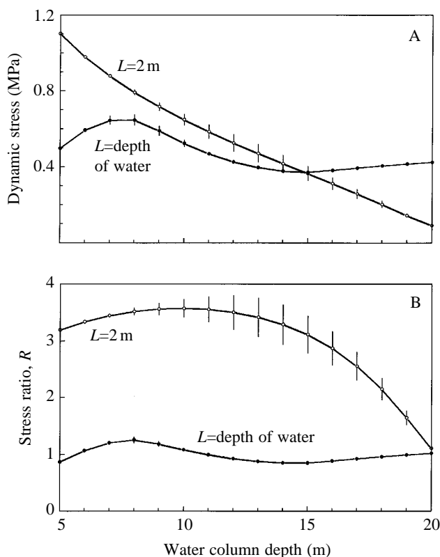
Fig. 19. The maximum dynamic stress (A) and maximum stress ratio (B) for allometric N. luetkeana as a function of the depth of the water column. Each point is the mean of values recorded in 50 wave cycles and the error bars are standard deviations, an index of the variation in each value. L , stipe length.
