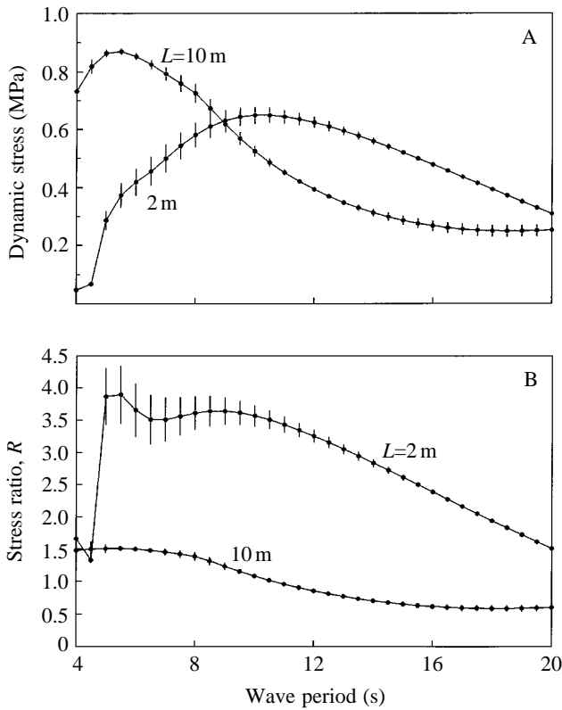
Fig. 11. The maximum stress (A) and maximum stress ratio (B) for N. luetkeana as a function of wave period. Each point is the mean of values recorded in 50 wave cycles and the error bars are standard deviations, an index of the variation in each value. L , stipe length.
