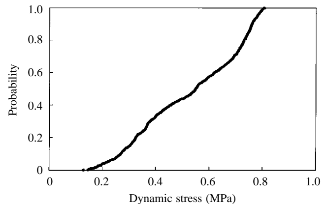
Fig. 21. The cumulative probability distribution of maximum stresses from 1500 wave cycles for a 'small'-shaped hypothetical plant undergoing chaotic motion.
