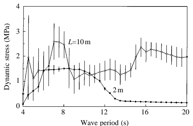
Fig. 18. Maximum stress as a function of wave period for hypothetical plants growing with the shape of a small N. luetkeana . Each point is the mean of values recorded in 50 wave cycles and the error bars are standard deviations, an index of the variation in each value. L , stipe length.
