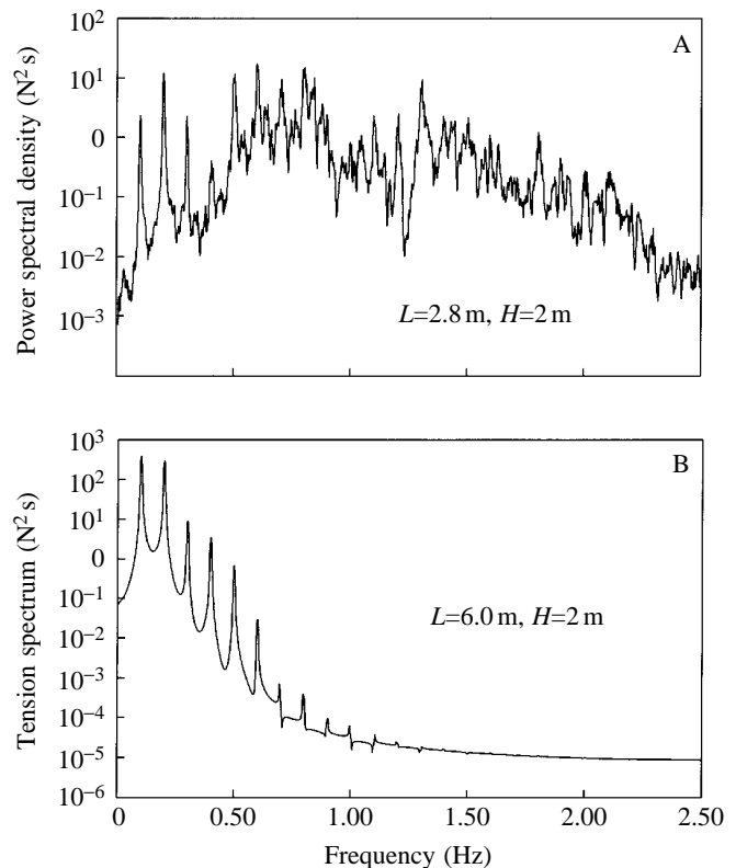
Fig. 15. (A) The power spectrum of tensions predicted by the numerical model for a hypothetical plants with a 'small' shape ( L=2.8\text{ m} , H=2\text{ m} , \tau=10\text{ s} , d=10\text{ m} ). The chaotic dynamics of the plant are evident in the noisy spectrum. (B) The power spectrum for a 'small'-shaped hypothetical plant under the same conditions as for A, but with L=6.0\text{ m} . The discrete peaks in B are indicative of periodic motion. L , stipe length; H , wave height; \tau , wave period; d , water column depth.
