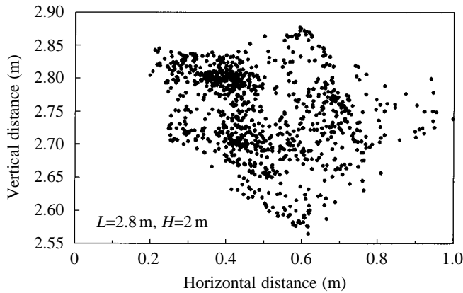
Fig. 16. A Poincaré section of the motion of a 'small'-shaped hypothetical plant ( H=2\text{ m} , \tau=10\text{ s} , d=10\text{ m} ) at an arbitrary phase in the wave cycle. The broad spread of points is indicative of chaos. L , stipe length; H , wave height; \tau , wave period; d , water column depth.
