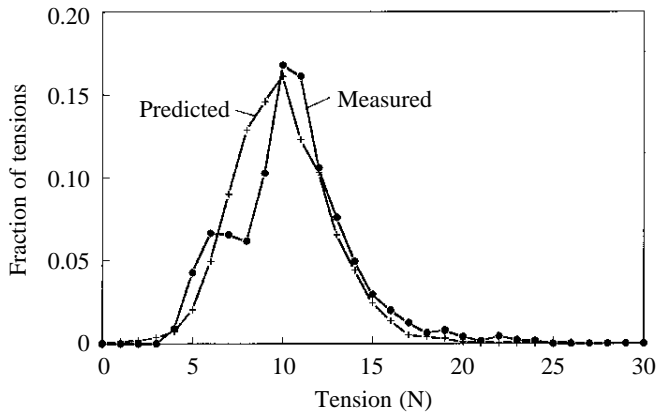
Fig. 4. A comparison of the distribution of stipe tensions recorded in the field (●) with those predicted by the numerical model (+). The mean measured tension is slightly higher than the mean predicted tension (see text).
