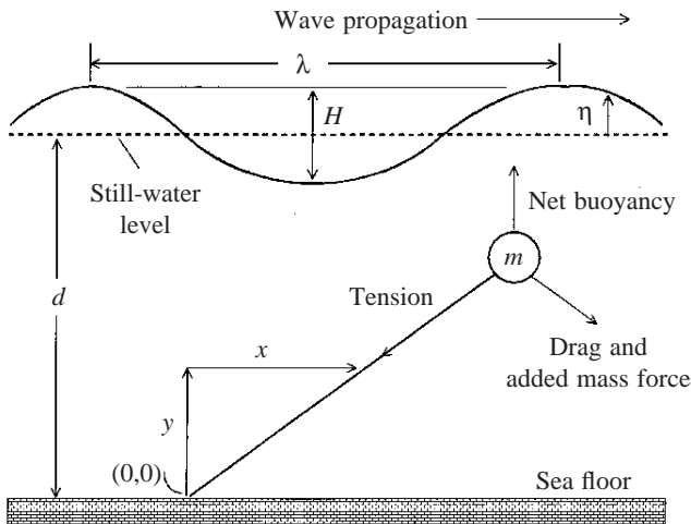
Fig. 2. A schematic representation of the numerical model of kelp dynamics. For further details, see the text. d , water column depth; H , wave height; \eta , vertical deviation from still-water level; m , plant mass; x , y , horizontal and vertical coordinate axes, respectively; \lambda , wavelength.
