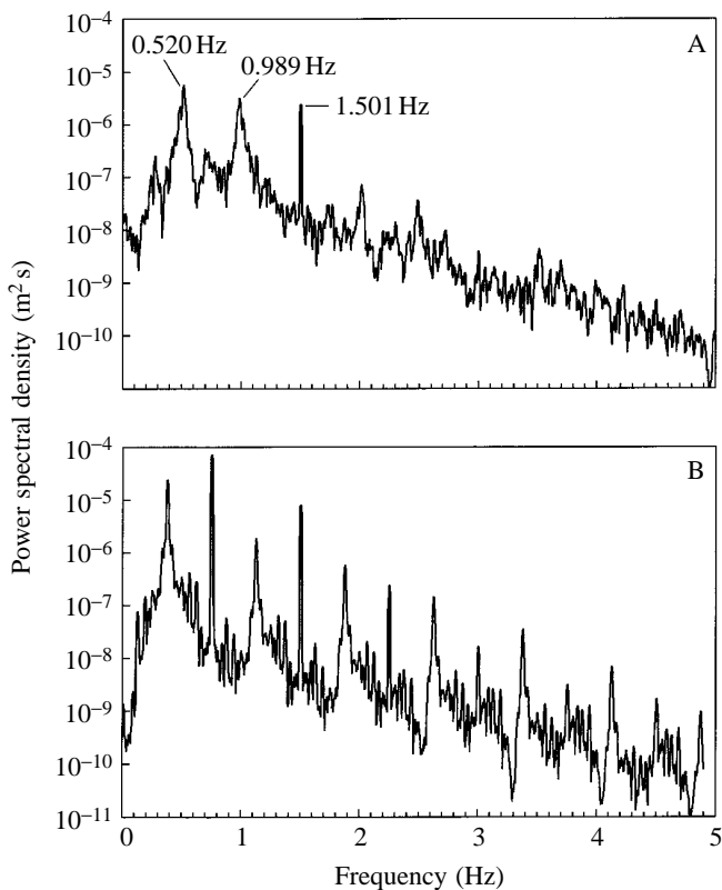
Fig. 8. The power spectra of y -directed motion of the corn-oil-filled ball in the wave tank (A) and in the numerical model (B). In each, there is a discrete peak at the driving frequency (1.50 Hz), but much of the variance in the ball's motion occurs at lower frequencies.
