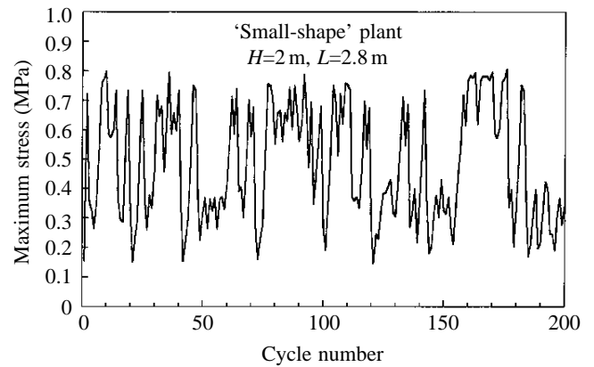
Fig. 20. A time series of the maximum stresses recorded in each of 200 wave cycles for a 'small'-shaped hypothetical plant undergoing chaotic motion. L , stipe length; H , wave height.
