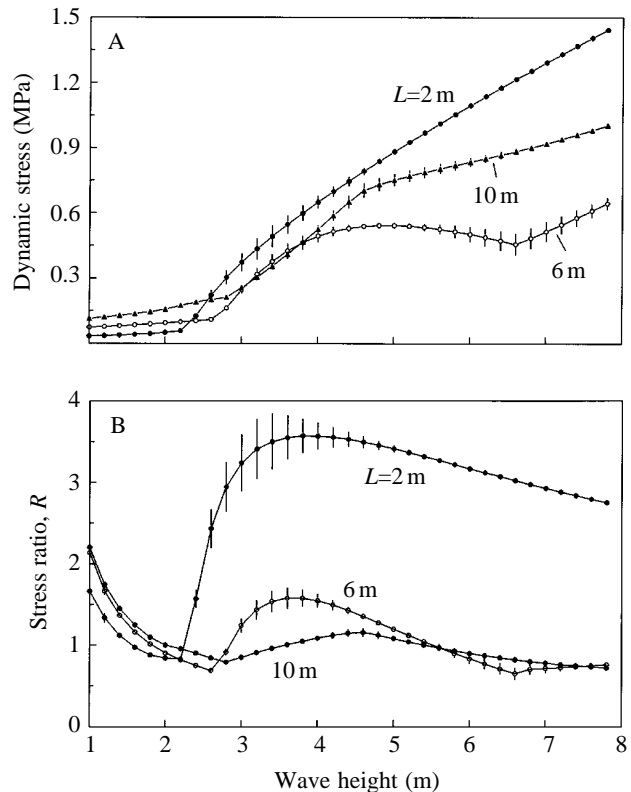
Fig. 10. The maximum stress (A) and maximum stress ratio (B) for N. luetkeana as a function of wave height. Each point is the mean of values recorded in 50 wave cycles and the error bars are standard deviations, an index of the variation in each value. L , stipe length.
