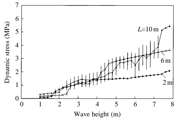
Fig. 17. Maximum dynamic stress as a function of wave height for hypothetical plants growing with the shape of a small N. luetkeana . Each point is the mean of values recorded in 50 wave cycles and the error bars are standard deviations, an index of the variation in each value. L , stipe length.
