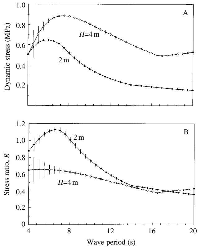
Fig. 13. The maximum stress (A) and maximum stress ratio (B) for mature N. luetkeana (stipe length L=10\text{ m} , with a threefold proliferation of blade area) as a function of wave period. Each point is the mean of values recorded in 50 wave cycles and the error bars are standard deviations, an index of the variation in each value. Depth 10\text{ m} . H , wave height.
