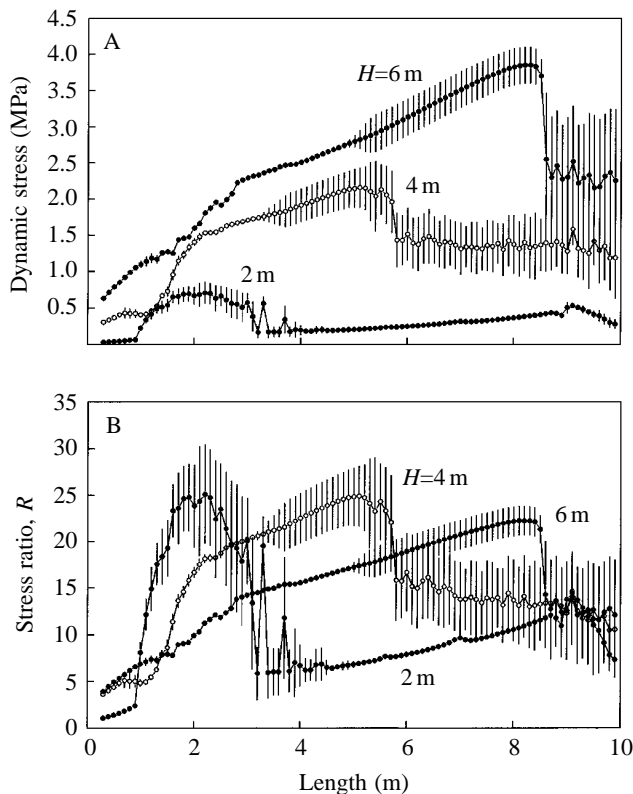
Fig. 14. The maximum stress (A) and maximum stress ratio (B) as a function of stipe length for hypothetical plants growing with the shape of a small (0.3 m long) N. luetkeana . Each point is the mean of values recorded in 50 wave cycles and the error bars are standard deviations, an index of the variation in each value. H , wave height.
