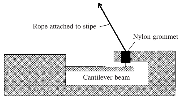
Fig. 3. A schematic representation of the force transducer used to measure the tension on a kelp stipe in the field. Strain gauges glued to the beam transduce the beam's deflection to a voltage that is recorded by the datalogger. The low-friction grommet ensures that the transducer senses the tension in the stipe regardless of the angle at which tension is applied.
