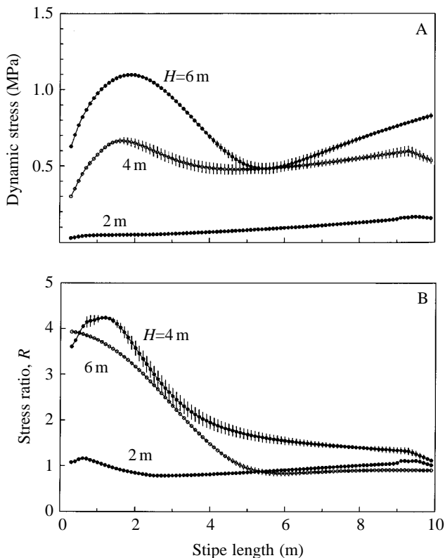
Fig. 9. The maximum stress (A) and maximum stress ratio (B) predicted for N. luetkeana as a function of stipe length. Each point is the mean of values recorded in 50 wave cycles and the error bars are standard deviations, an index of the variation in each value. H , wave height.
