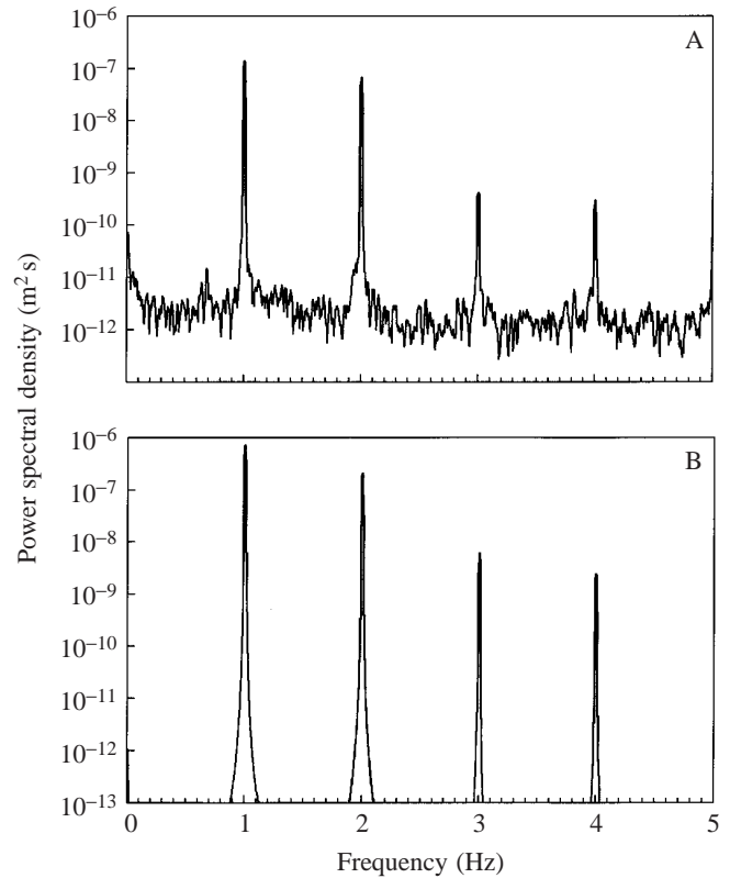
Fig. 6. The power spectra of (A) y -directed motion recorded in the wave tank for the air-filled ball and (B) y -directed motion predicted by the numerical model. The spectra from x -directed motion in the physical and numerical models show a similar match.
