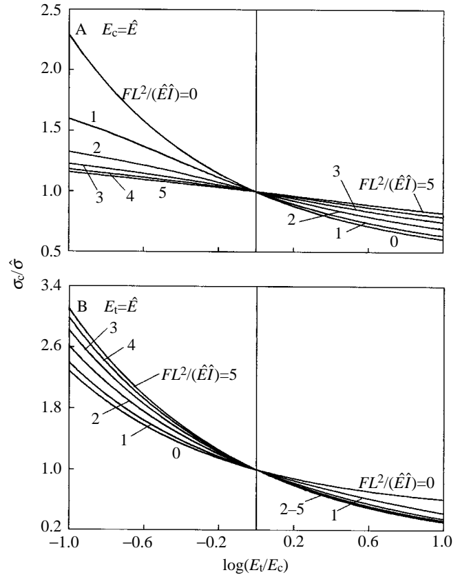
Fig. 15. Effects on the compressive stress of having unequal moduli, as a function of the nondimensionalized force, FL^2/(\hat{E}\hat{I}) . Compressive stresses decline with larger E_t/E_c ratios either for E_c=\hat{E} (A) or for E_t=\hat{E} (B). \hat{\sigma} and \hat{E}\hat{I} are the tensile stress and effective flexural stiffness, respectively, computed when E_t=E_c=\hat{E} . \sigma/\hat{\sigma} is the ratio of the altered to the original stress.
